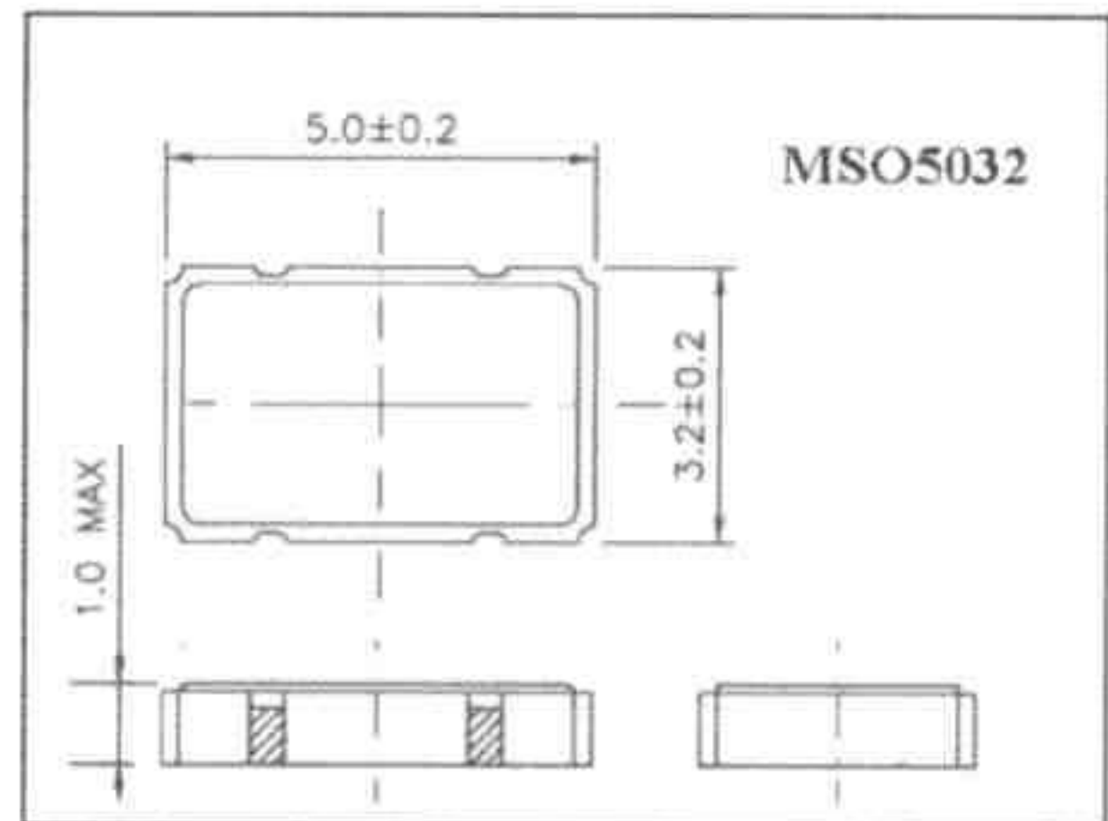
External Dimension (Unit: mm)
